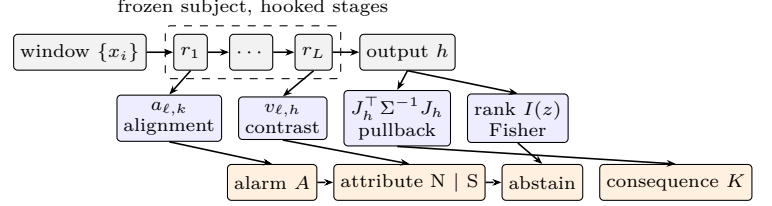
Figure 1: Monitor stack on a frozen subject. Hooked stages feed two gauge-safe layerwise statistics (alignment a_{\ell,k} , contrastive direction v_{\ell,h} ); the output map feeds the pullback metric and the Fisher rank. Alarm, N/S attribution, abstention, and the consequence measure K are separate endpoints with separate false-alert budgets, and every arrow is a pre-registered prediction on Tier 1 before Tier 2 runs.
